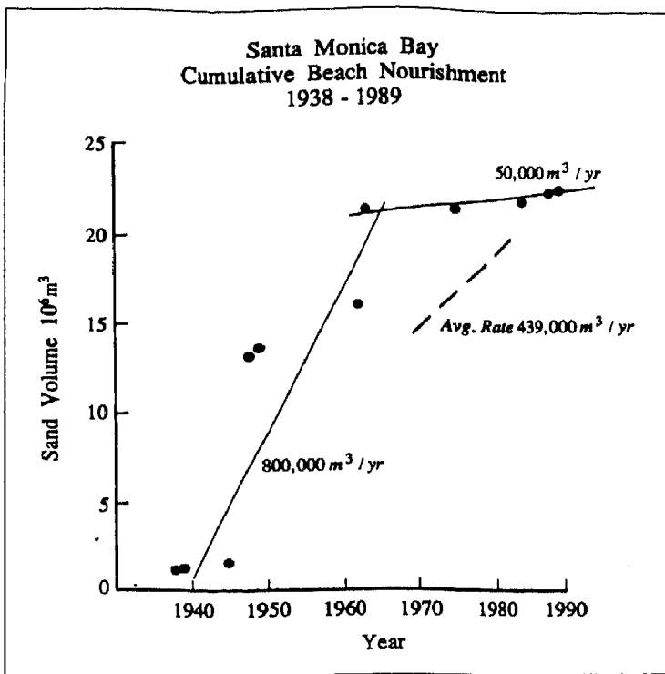
Fig. 3 Cumulative beach sand nourishment in the Santa Monica Bay littoral cell. Nourishment rates have decreased considerably since 1963, when the last dredge spoils from Marina del Rey were placed on Dockweiler Beach, but the overall annualized rate (dashed) still far exceeds that of natural or actual river sand supply.
